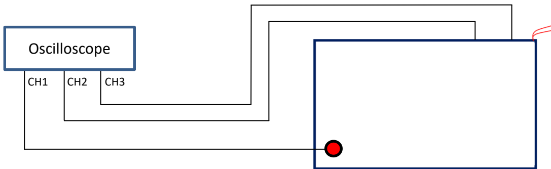
Figure 1: Test setup
